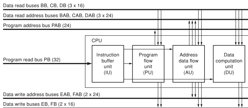
Figure D.4 Architecture of the TMS320C55 DSP. The C55 is a seven-stage pipelined processor with some unique instruction execution facilities. (Courtesy Texas Instruments.)
