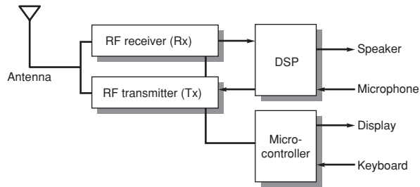
Figure D.16 Block diagram of a cell phone. The DSP performs the signal processing steps of Figure D.15, and the microcontroller controls the user interface, battery management, and call setup. (Based on Figure 1.3 of Groe and Larson [2000].)
