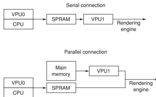
Figure D.12 Two modes of using Emotion Engine organization. The first mode divides the work between the two units, and then allows the Graphics Interface to properly merge the display lists. The second mode uses CPU/VPU0 as a filter of what to send to VPU1, which then does all the display lists. It is up to the programmer to choose between serial and parallel data flow. SPRAM is the scratchpad memory.
