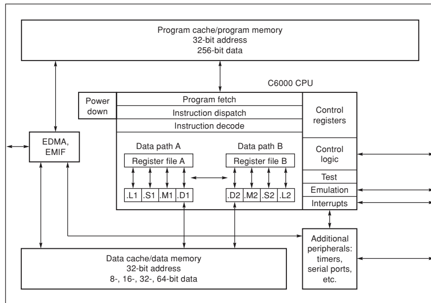
Figure D.5 Architecture of the TMS320C64x family of DSPs. The C6x is an eight-issue traditional VLIW processor. (Courtesy Texas Instruments.)
