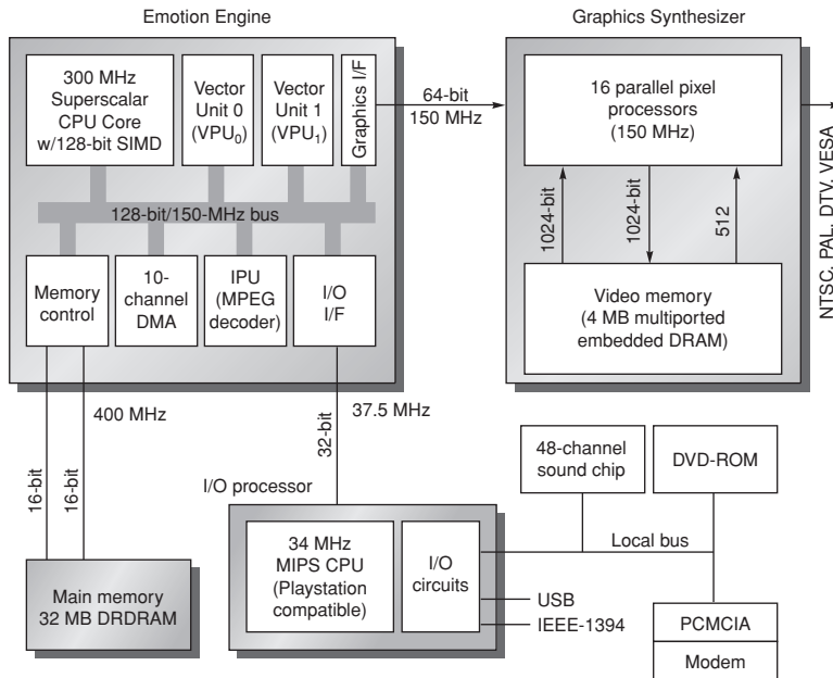
Figure D.11 Block diagram of the Sony Playstation 2. The 10 DMA channels orchestrate the transfers between all the small memories on the chip, which when completed all head toward the Graphics Interface so as to be rendered by the Graphics Synthesizer. The Graphics Synthesizer uses DRAM on chip to provide an entire frame buffer plus graphics processors to perform the rendering desired based on the display commands given from the Emotion Engine. The embedded DRAM allows 1024-bit transfers between the pixel processors and the display buffer. The Superscalar CPU is a 64-bit MIPS III with two-instruction issue, and comes with a 2-way set-associative, 16 KB instruction cache; a 2-way set-associative, 8 KB data cache; and 16 KB of scratchpad memory. It has been extended with 128-bit SIMD instructions for multimedia applications (see Section D.2). Vector Unit 0 is primarily a DSP-like coprocessor for the CPU (see Section D.2), which can operate on 128-bit registers in SIMD manner between 8 bits and 32 bits per word. It has 4 KB of instruction memory and 4 KB of data memory. Vector Unit 1 has similar functions to VPU 0 , but it normally operates independently of the CPU and contains 16 KB of instruction memory and 16 KB of data memory. All three units can communicate over the 128-bit system bus, but there is also a 128-bit dedicated path between the CPU and VPU 0 and a 128-bit dedicated path between VPU 1 and the Graphics Interface. Although VPU 0 and VPU 1 have identical microarchitectures, the differences in memory size and units to which they have direct connections affect the roles that they take in a game. At 0.25-micron line widths, the Emotion Engine chip uses 13.5M transistors and is 225 mm 2 , and the Graphics Synthesizer is 279 mm 2 . To put this in perspective, the Alpha 21264 microprocessor in 0.25-micron technology is about 160 mm 2 and uses 15M transistors. (This figure is based on Figure 1 in "Sony's Emotionally Charged Chip," Microprocessor Report 13:5.)
