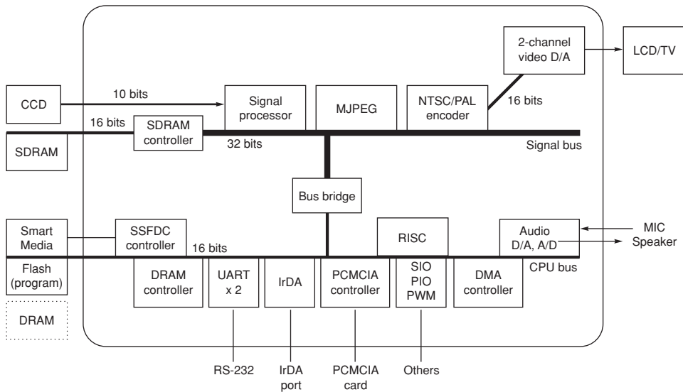
Figure D.13 The system on a chip (SOC) found in Sanyo digital cameras. This block diagram, found in Okada et al. [1999], is for the predecessor of the SOC in the camera described in the text. The successor SOC, called Super Advanced IC, uses three buses instead of two, operates at 60 MHz, consumes 800 mW, and fits 3.1M transistors in a 10.2 x 10.2 mm die using a 0.35-micron process. Note that this embedded system has twice as many transistors as the state-of-the-art, high-performance microprocessor in 1990! The SOC in the figure is limited to processing 1024 x 768 pixels, but its successor supports 1360 x 1024 pixels.
