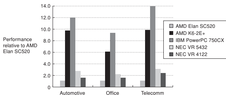
Figure D.10 Raw performance for the five embedded processors. The performance is presented as relative to the performance of the AMD ElanSC520.
