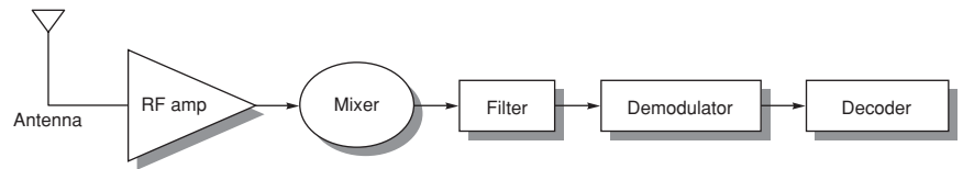
Figure D.15 A radio receiver consists of an antenna, radio frequency amplifier, mixer, filters, demodulator, and decoder. A mixer accepts two signal inputs and forms an output signal at the sum and difference frequencies. Filters select a narrower band of frequencies to pass on to the next stage. Modulation encodes information to make it more robust. Decoding turns signals into information. Depending on the application, all electrical components can be either analog or digital. For example, a car radio is all analog components, but a PC modem is all digital except for the amplifier. Today analog silicon chips are used for the RF amplifier and first mixer in cellular phones.
